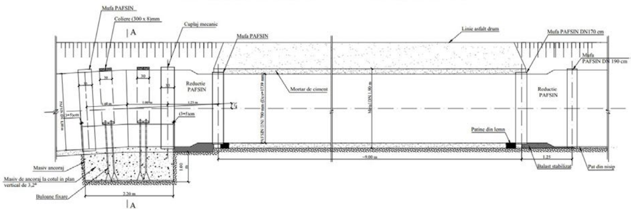
Fig. 22 Under-crossing and thrust block for the elbows in vertical plane
