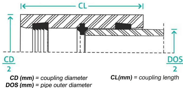
Fig. 26 Sketch of a Reka coupling connected to a GRP pipe
