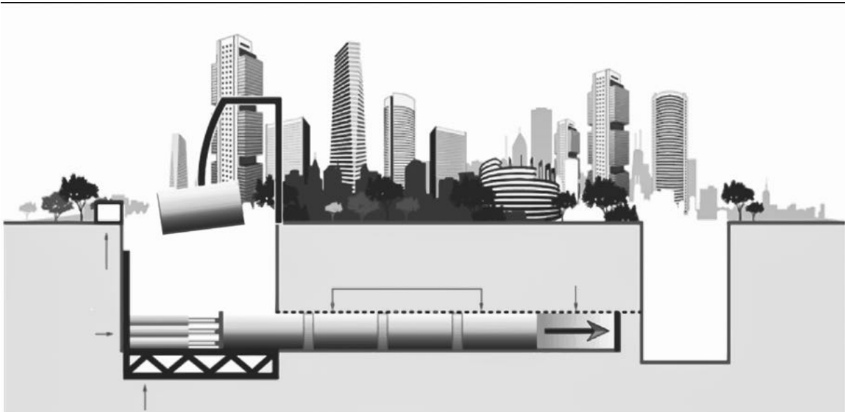
Fig. 21 Pipe jacking process sketch
